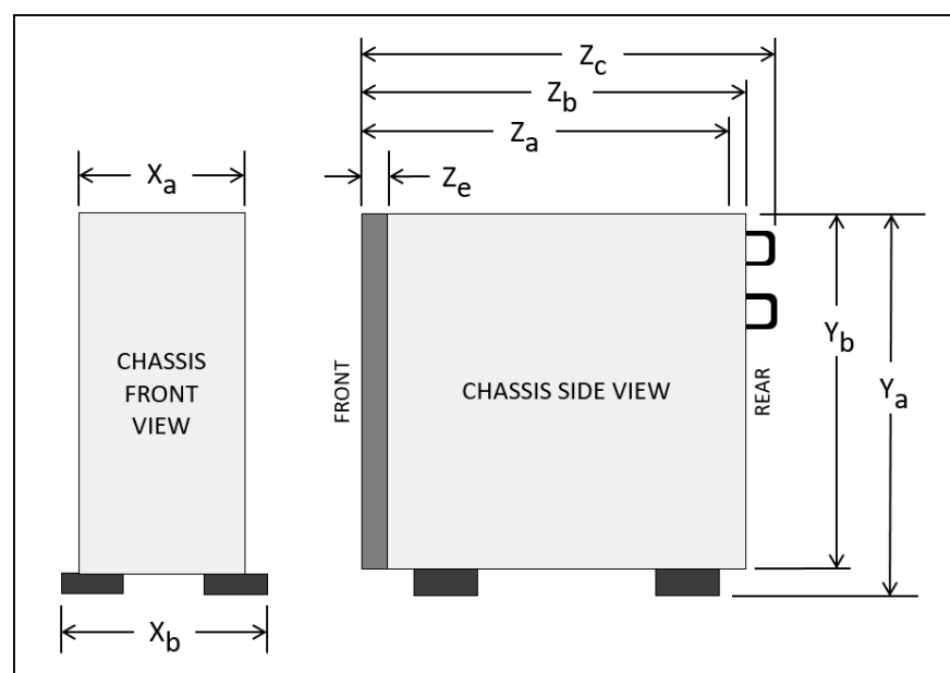
Figure 10. Server dimension
